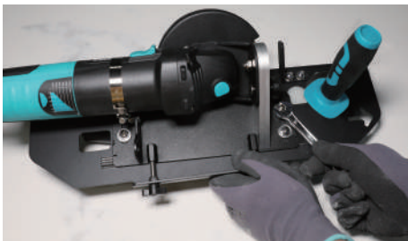
Step 3. Tighten the scews
