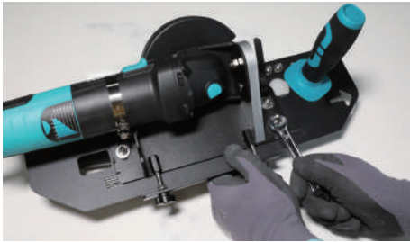
Step 1. Loose three screws
