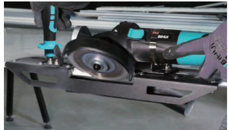
Step 2. Keep the bearing close leaning and sliding on the edge of tile (slab)
