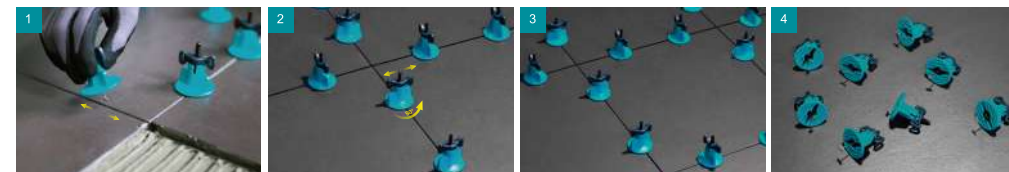
1. Insert T-pin parallel into the grout joint (For a wider joint, use classic spacers together) 2. Hold the blue cap in 90° position and spin down the gray handle 3. Twist the gray handle down to the required level (no tools needed) 4. Return parallel back for 90° to the grout joint for reuse (Note: remove within 24 hrs)*
