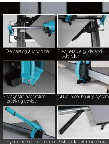
1.Die casting support bar 2.Adjustable guide and side ruler 3.Magnetic absorption breaking device 4.Built-in ball bearing system 5.Ergonomic soft grip handle 6.Movable extension bars
