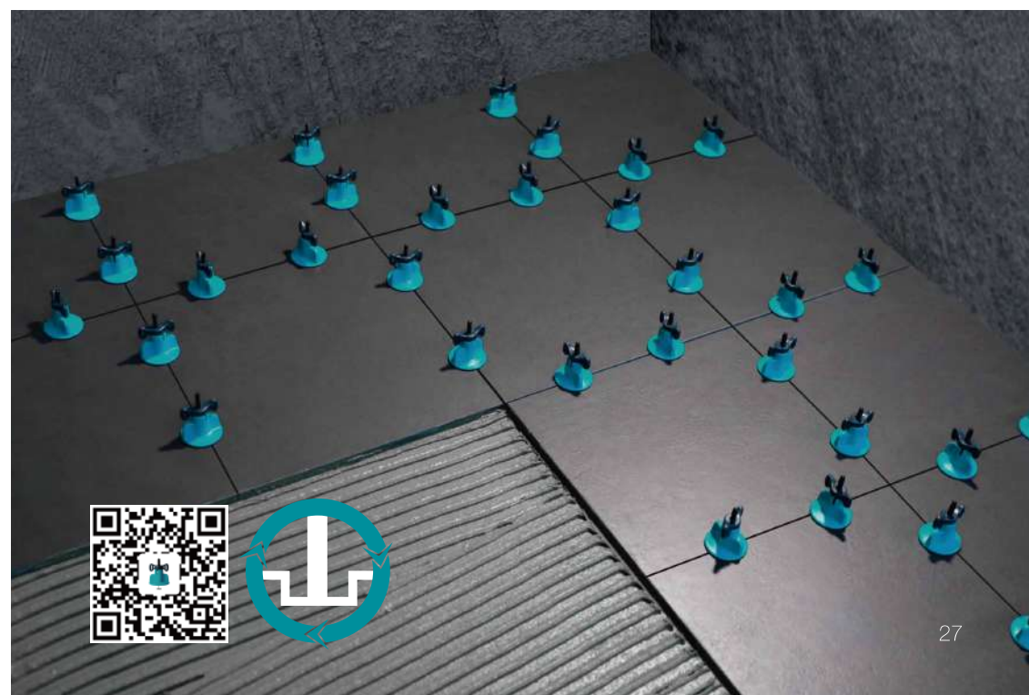
1. Insert T-pin parallel into the grout joint (For a wider joint, use classic spacers together) 2. Hold the blue cap in 90° position and spin down the gray handle 3. Twist the gray handle down to the required level (no tools needed) 4. Return parallel back for 90° to the grout joint for reuse (Note: remove within 24 hrs)*
