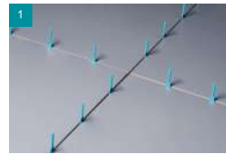
1 Place the level base under the tiles 10 cm from either end
